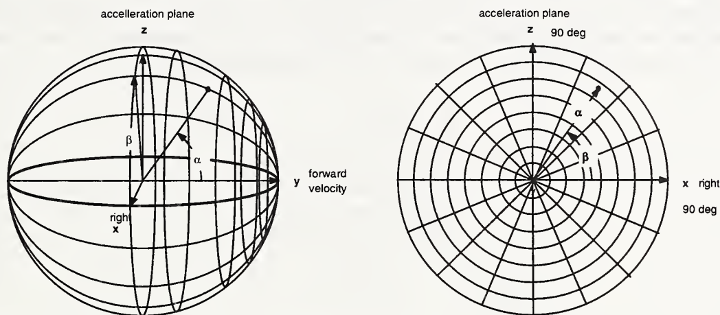
Figure 24. Two views of a velocity egosphere. On the left is a perspective view from the upper right side. On the right is a view along the velocity vector from the center. The velocity vector defines the pole of the velocity egosphere, and that corresponds to the focus of expansion of flow vectors for stationary points in the image.
